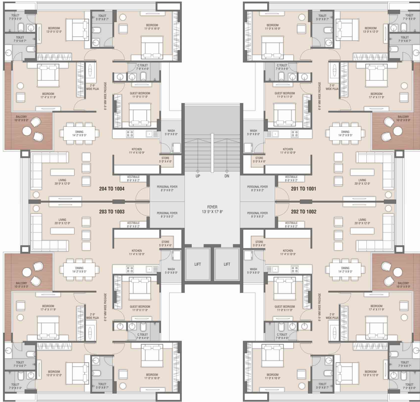
TYPICAL FLOOR PLAN (2nd TO 10th)
